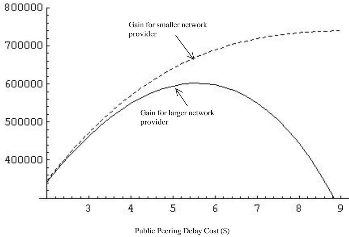
Figure 7: Impact of Public Peering Point Congestion
