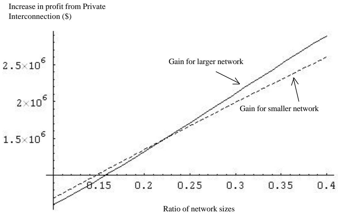
Figure 4: Increase in profits from Private Interconnection agreements Vs. Relative network sizes
