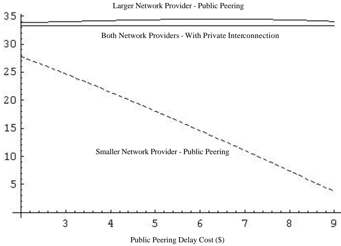
Figure 5: Impact of Peering Point Congestion on Market Coverage
